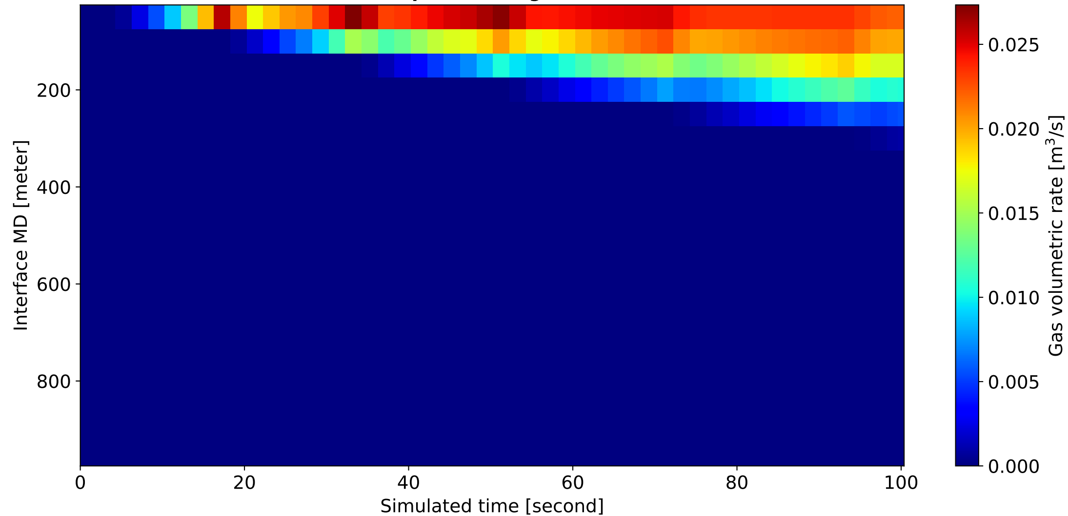
Gas volumetric rate profile along the wellbore over time
